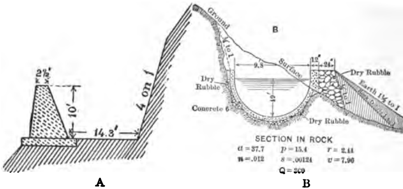
FIG. 67.—Rock Cross-section; Umatilla Canal.
